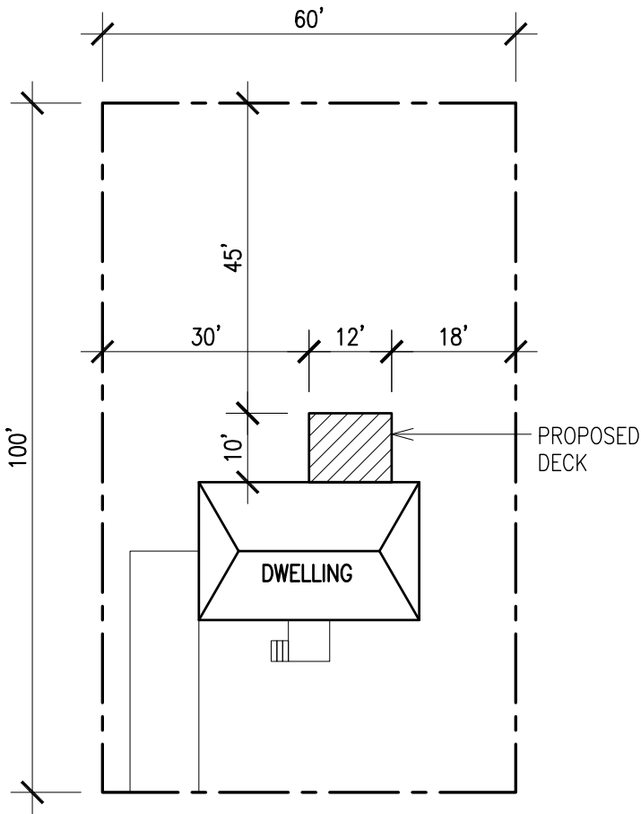
SITE PLAN EXAMPLE – PROPOSED DECK
