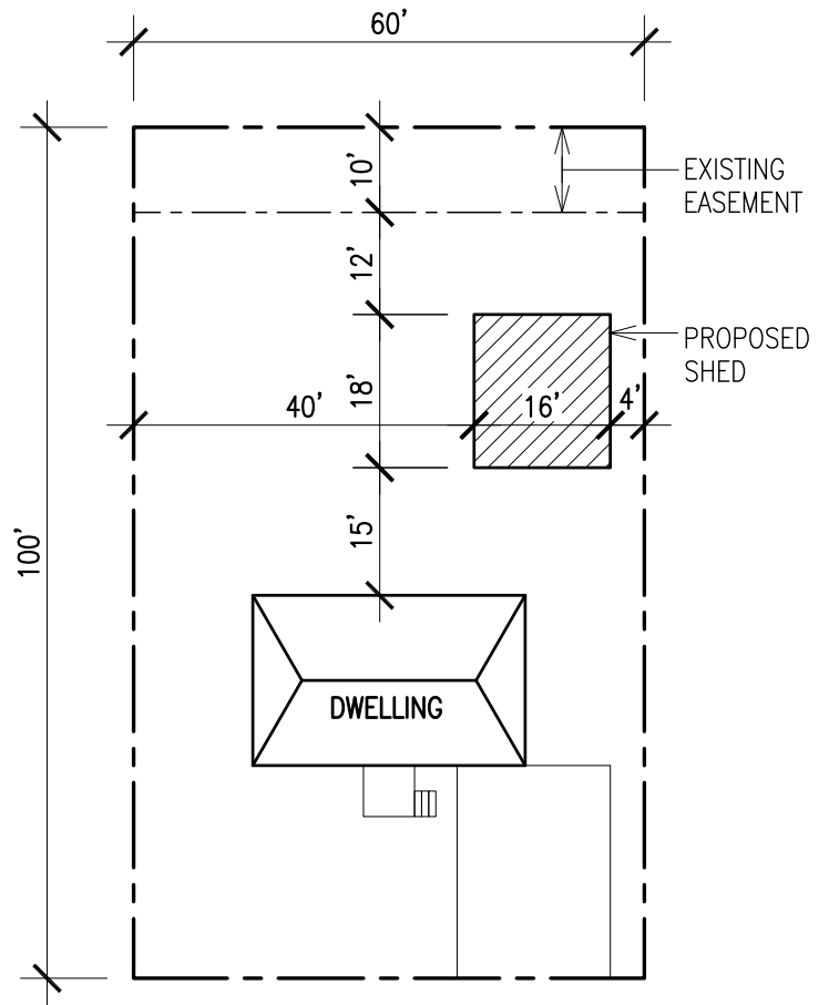
SITE PLAN EXAMPLE – PROPOSED SHED
