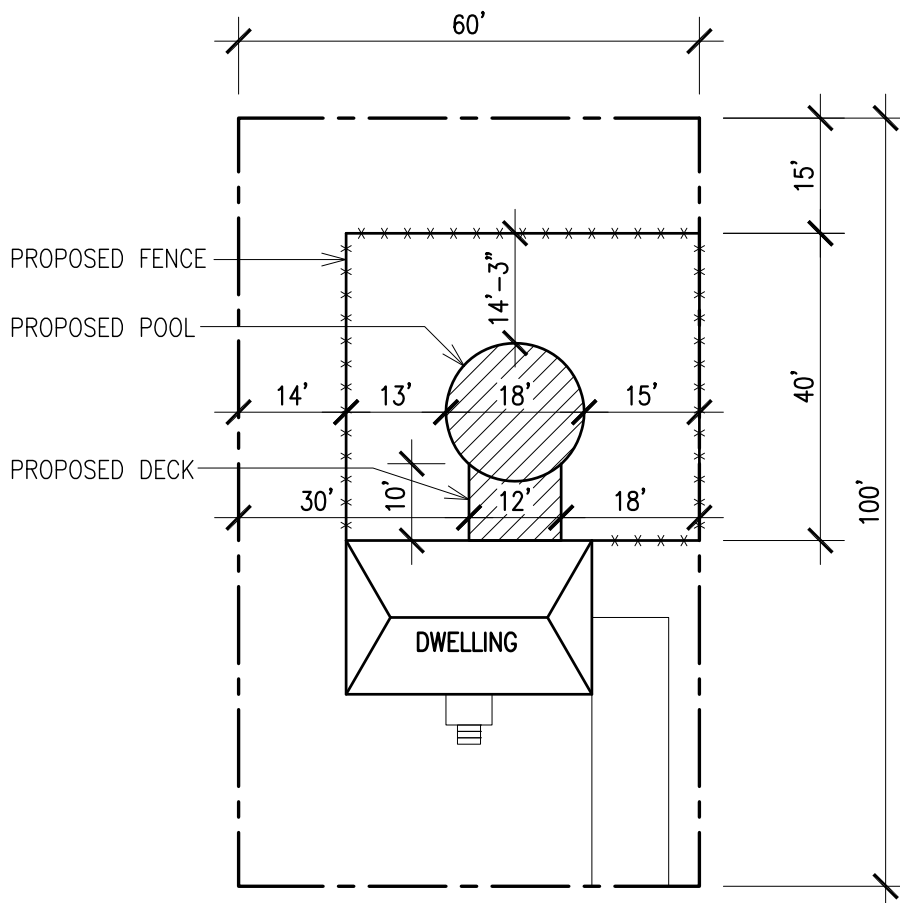
SITE PLAN EXAMPLE – PROPOSED POOL, DECK & FENCE
